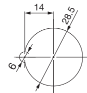
Plate thickness VHL21□W: Max. 3.5
