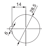
Plate thickness VHL212S: Max. 3.5
