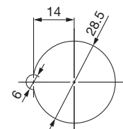
Panel cutout dimensions
