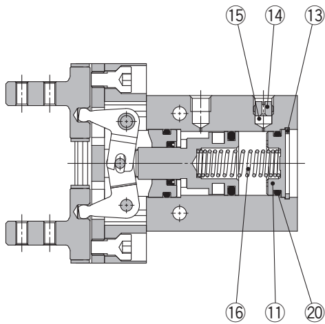
Single acting, Normally open
