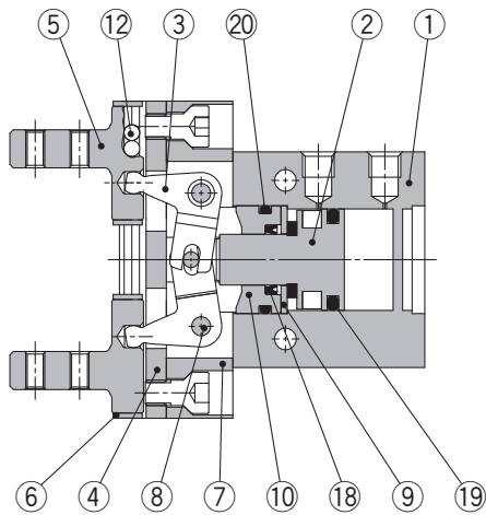
Double acting, With fingers open
