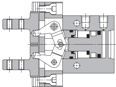
Double acting, With fingers closed
