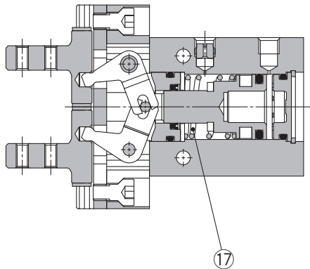
Single acting, Normally closed
